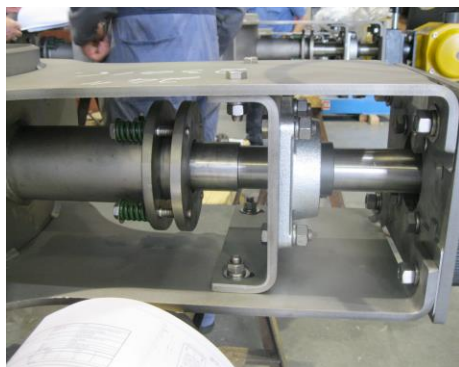
Flange Mounted External Bearings. Packing Gland and Lantern Ring Design c/w Air Purge
