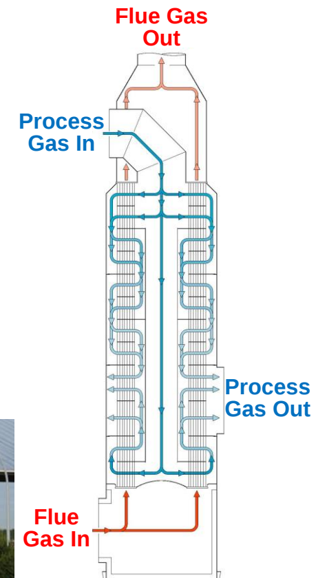
NORAM RF™ SF™ preheat exchanger
