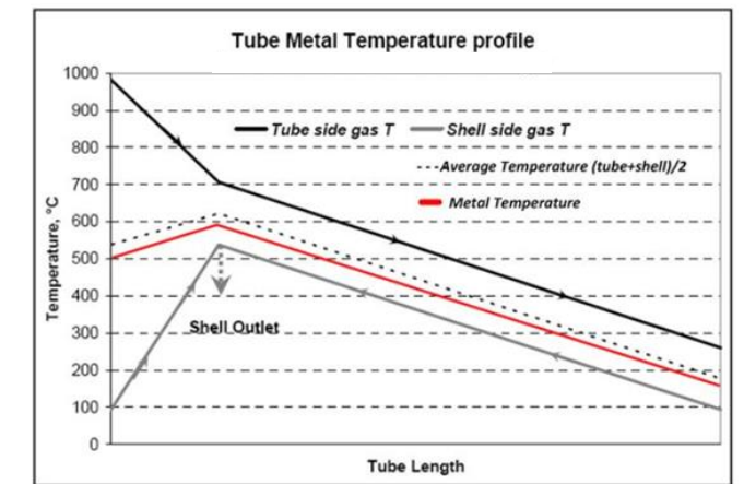
NORAM RF™ SF™ preheat exchanger
