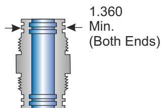
Tandem Sub
